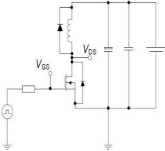
Unclamped inductive load test circuit waveform
